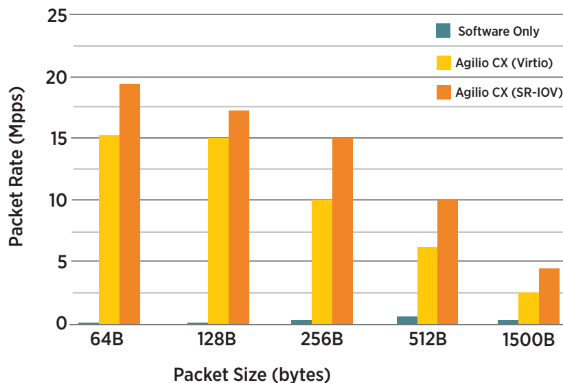
Bi-Directional Agilio CX- 40GbE - Nuage VSP
